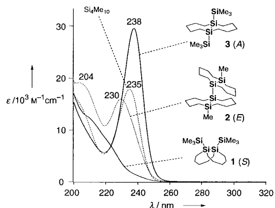
Figure 1. UV absorption spectra of the tetrasilane compounds 1–3 and \text{Si}_4\text{Me}_{10} .
